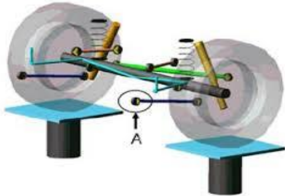
Figure A: Half car model with 5-link rear suspension
