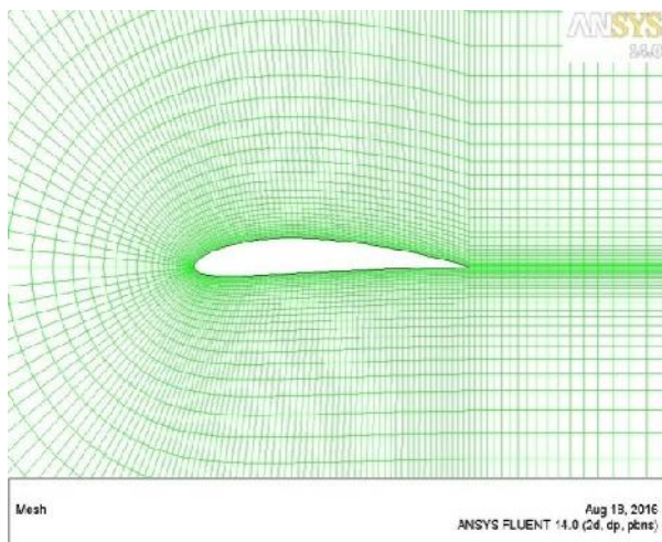
Figure 1:- (a) Meshing of the airfoil, (b) Zoom view of the meshing
